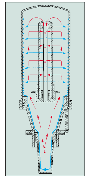
Recombination principle in the AquaGen® vent plug D 48. - Gas - Water
